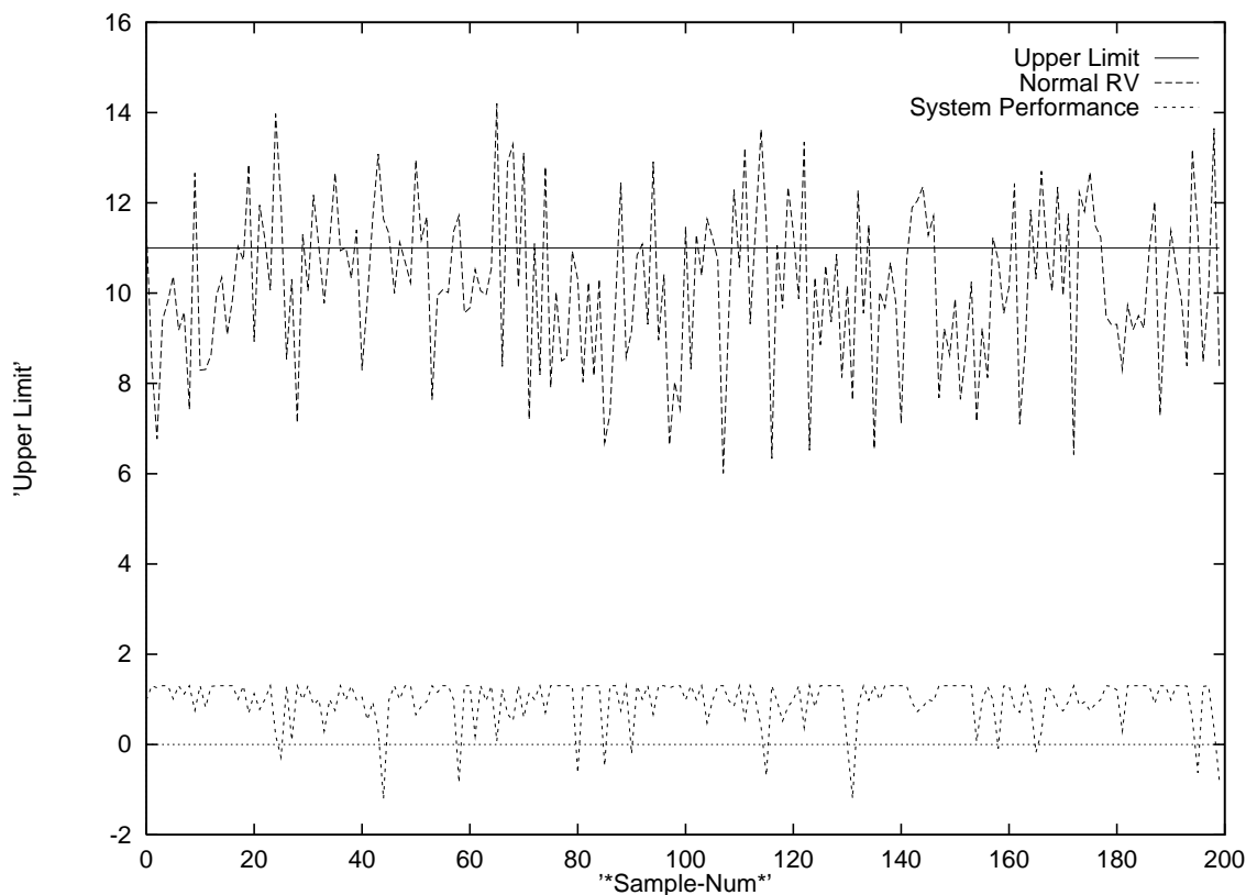
Fig. 13. System Performance.
